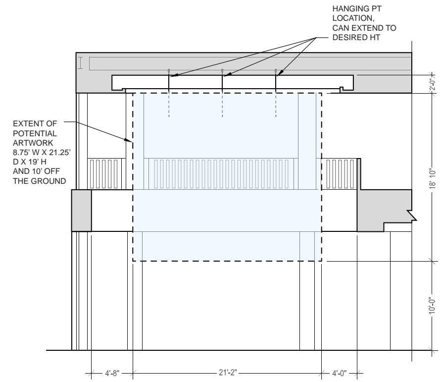
[03] SECTION DIAGRAM 3/32" = 1'
