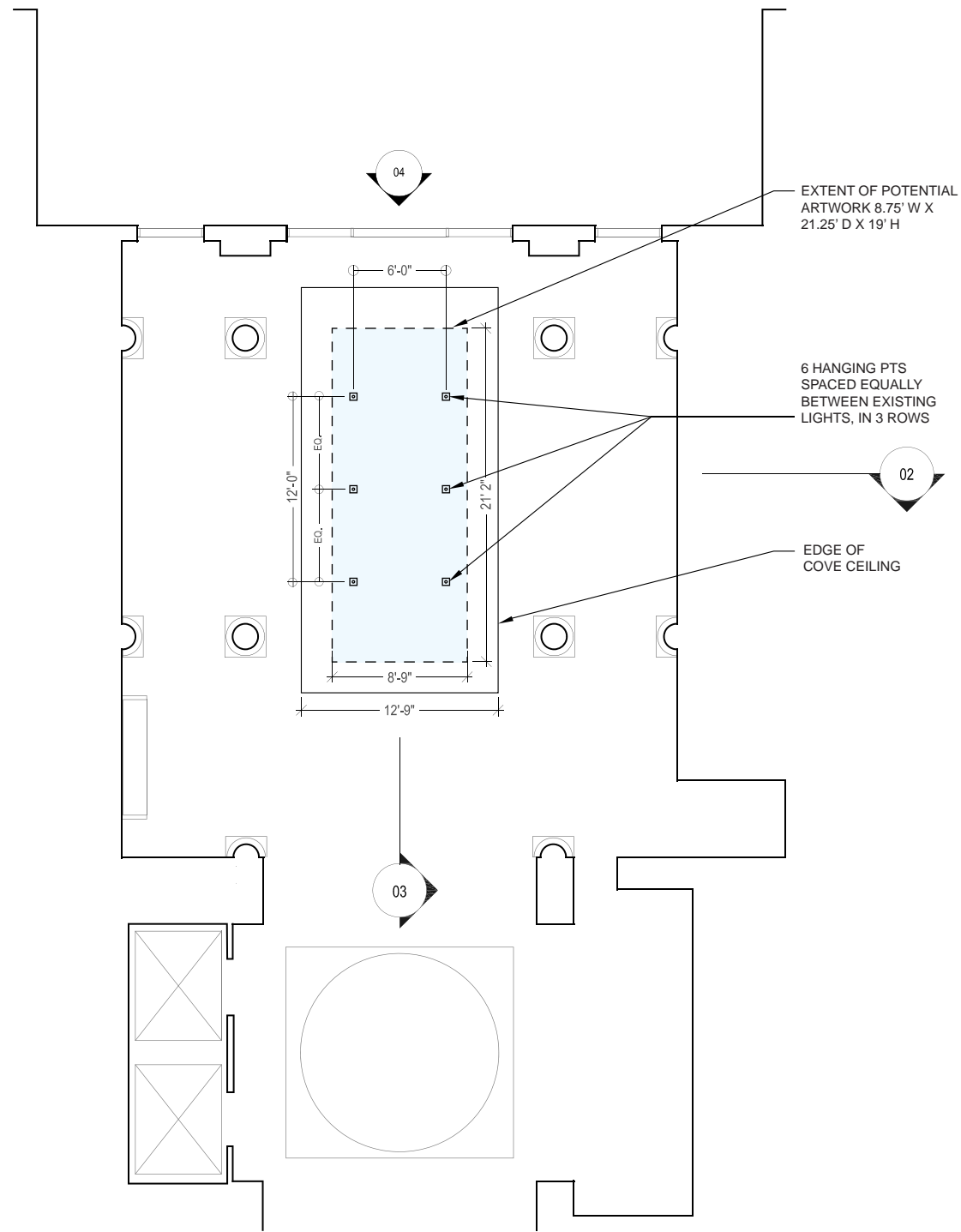
[01] RCP DIAGRAM 3/32" = 1'
