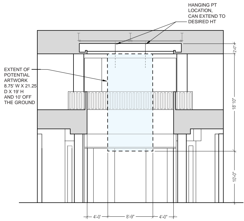
[02] SECTION DIAGRAM 3/32" = 1'
