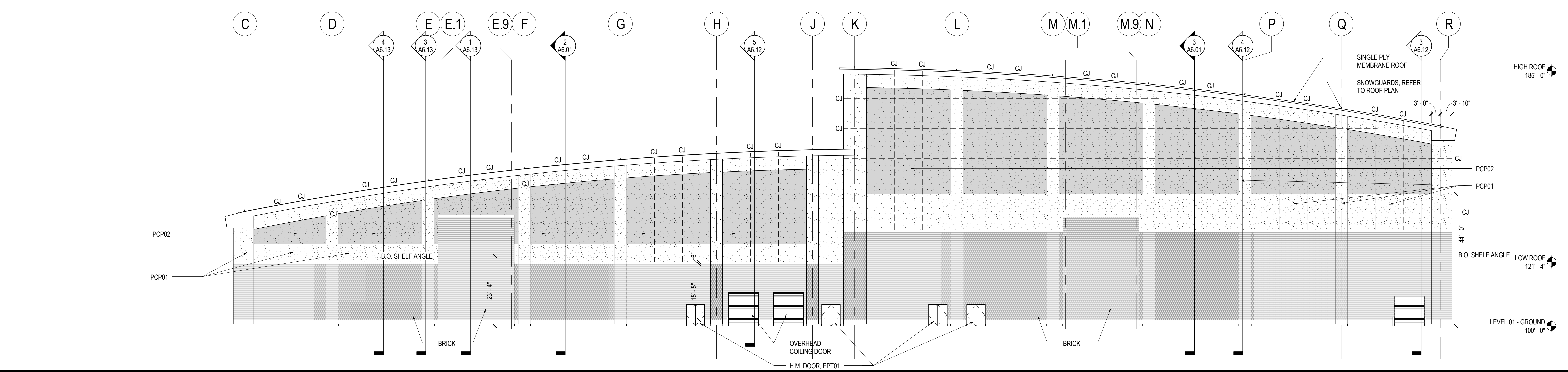
3 BUILDING ELEVATION - SOUTH SCALE: 1/16" = 1'-0"
