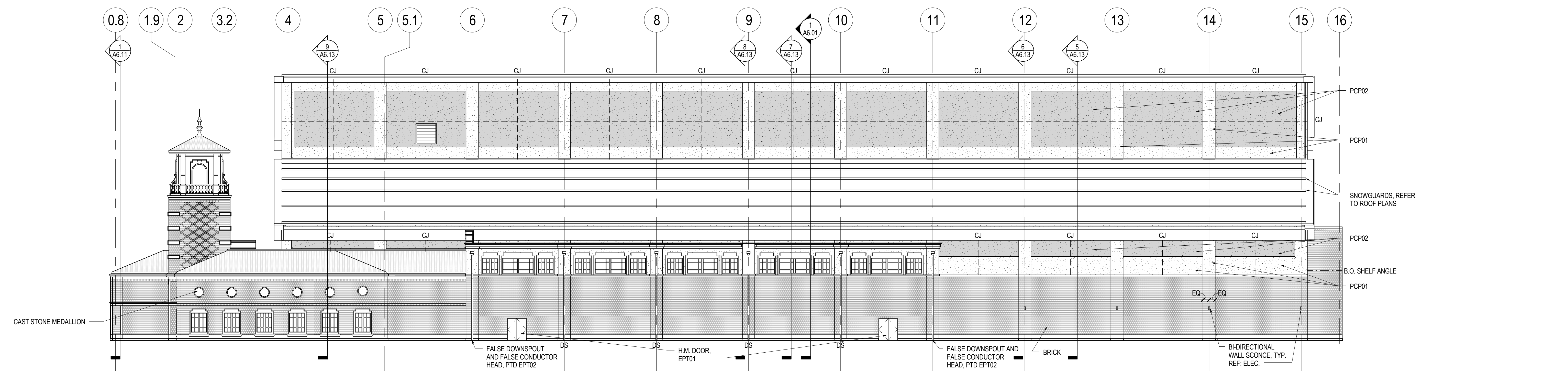
4 BUILDING ELEVATION - WEST SCALE: 1/16" = 1'-0"
