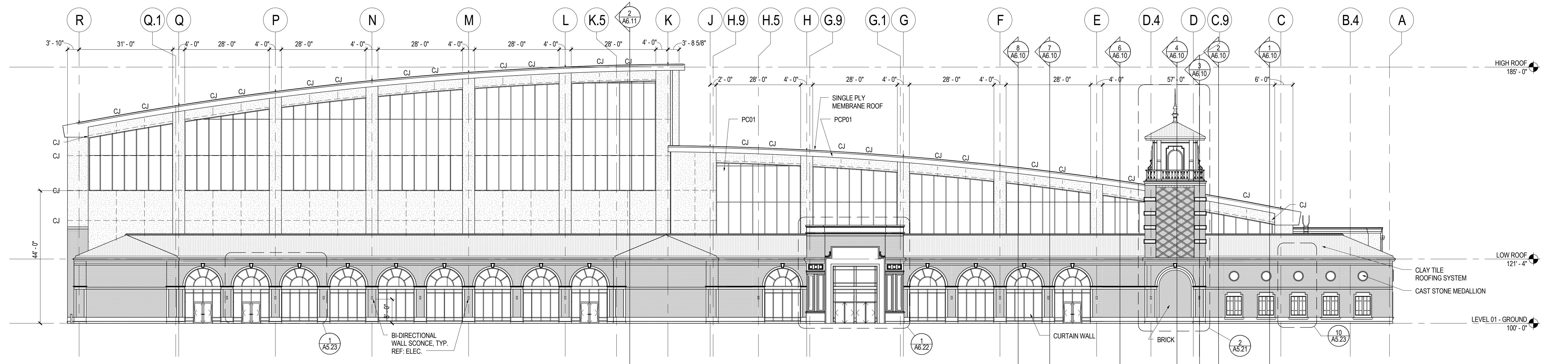
1 BUILDING ELEVATION - NORTH SCALE: 1/16" = 1'-0"
